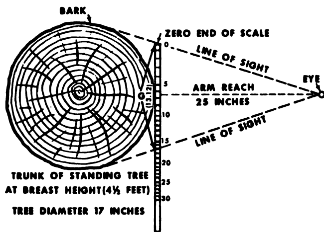
Figure 2-8. Biltmore stick.
